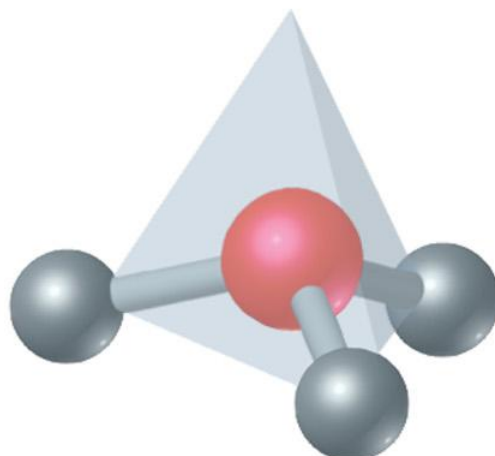
Trigonal pyramidal
