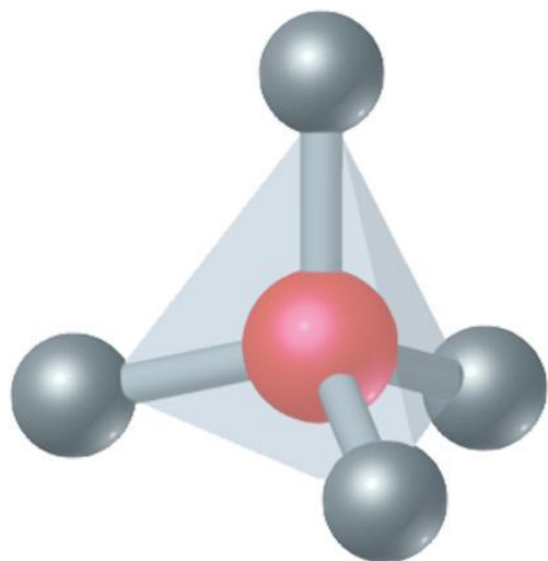
Tetrahedral
