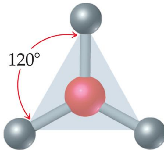
Trigonal planar
