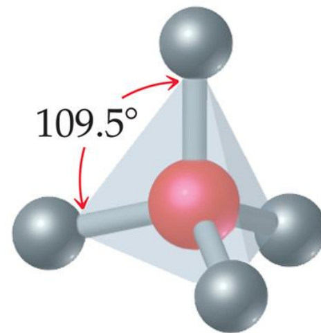
Tetrahedral
